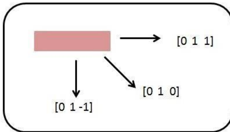
Figure 2: Reciprocal lattice
